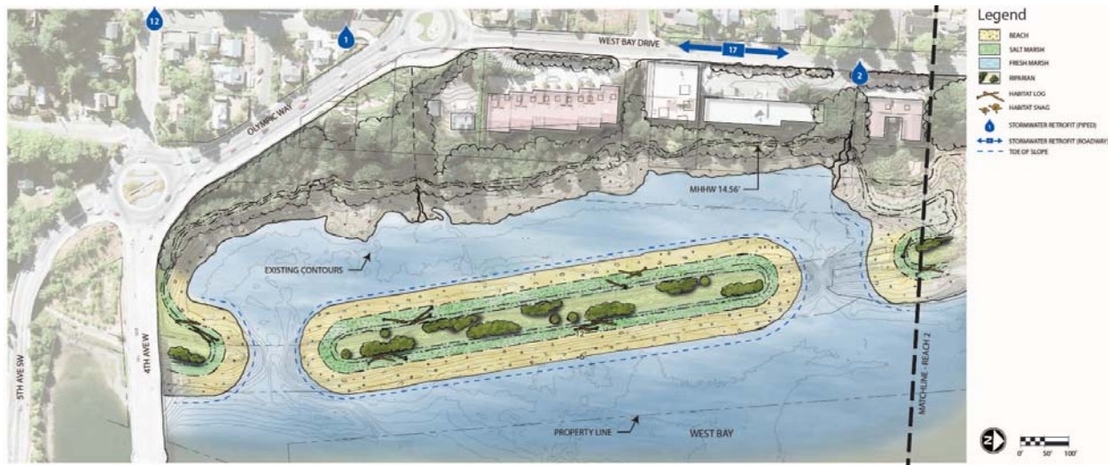
Figure 2. Lagoon Alternative 1.
