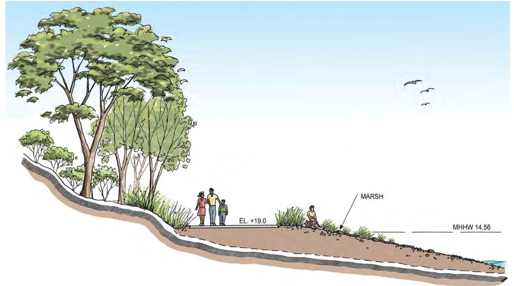
Conceptual Section 6
