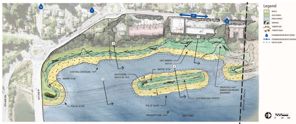
Figure 4. Lagoon Alternative 3.
