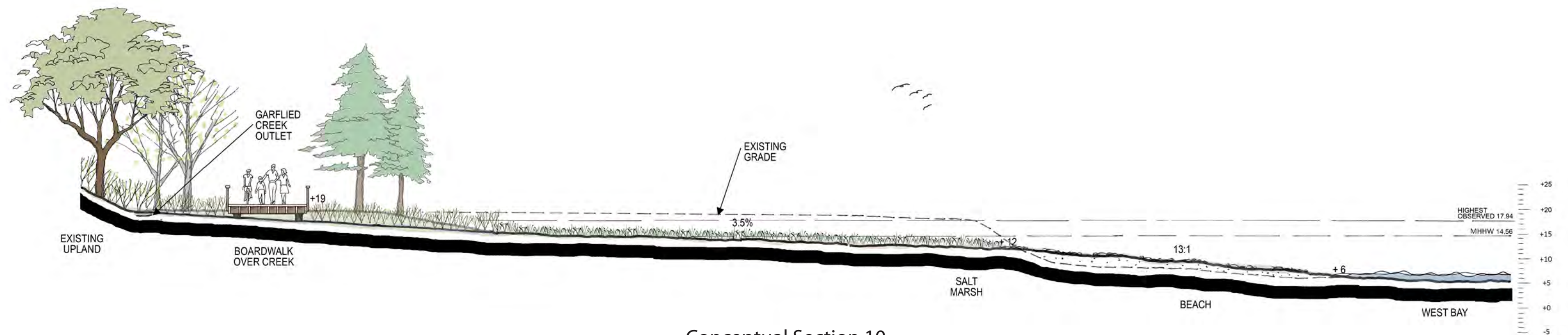
Conceptual Section 10
