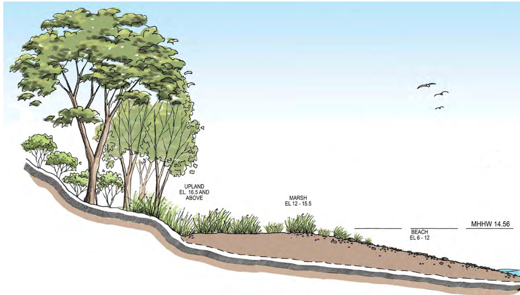
Conceptual Section 3
