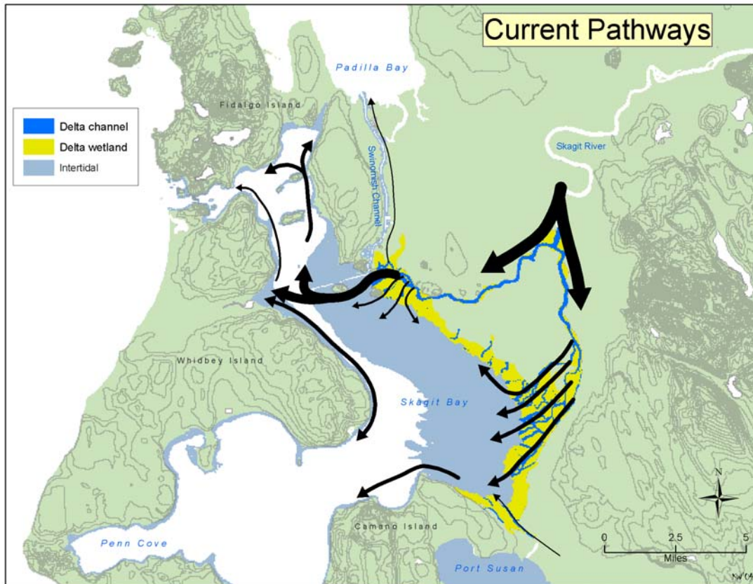
Figure 2. Current juvenile Chinook salmon migration pathways in the Skagit delta. The arrow directions depict how juvenile Chinook salmon move through delta habitat and into Skagit Bay. Arrow thickness represents the number of juvenile Chinook salmon using each pathway based on current habitat amount and configuration. Wider arrows represent more fish than narrow arrows.
