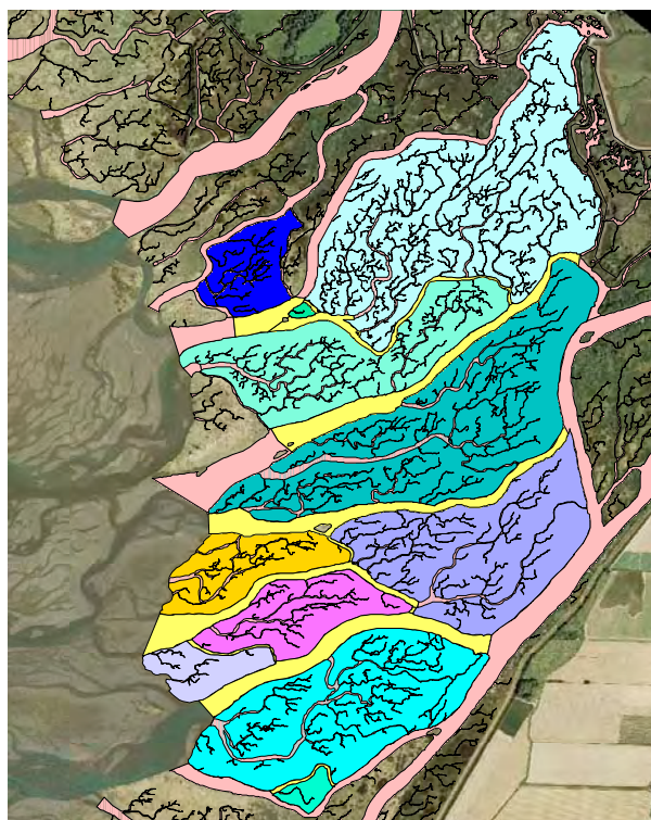
Figure 2.6 – Marsh Islands for the South Fork Skagit Delta
