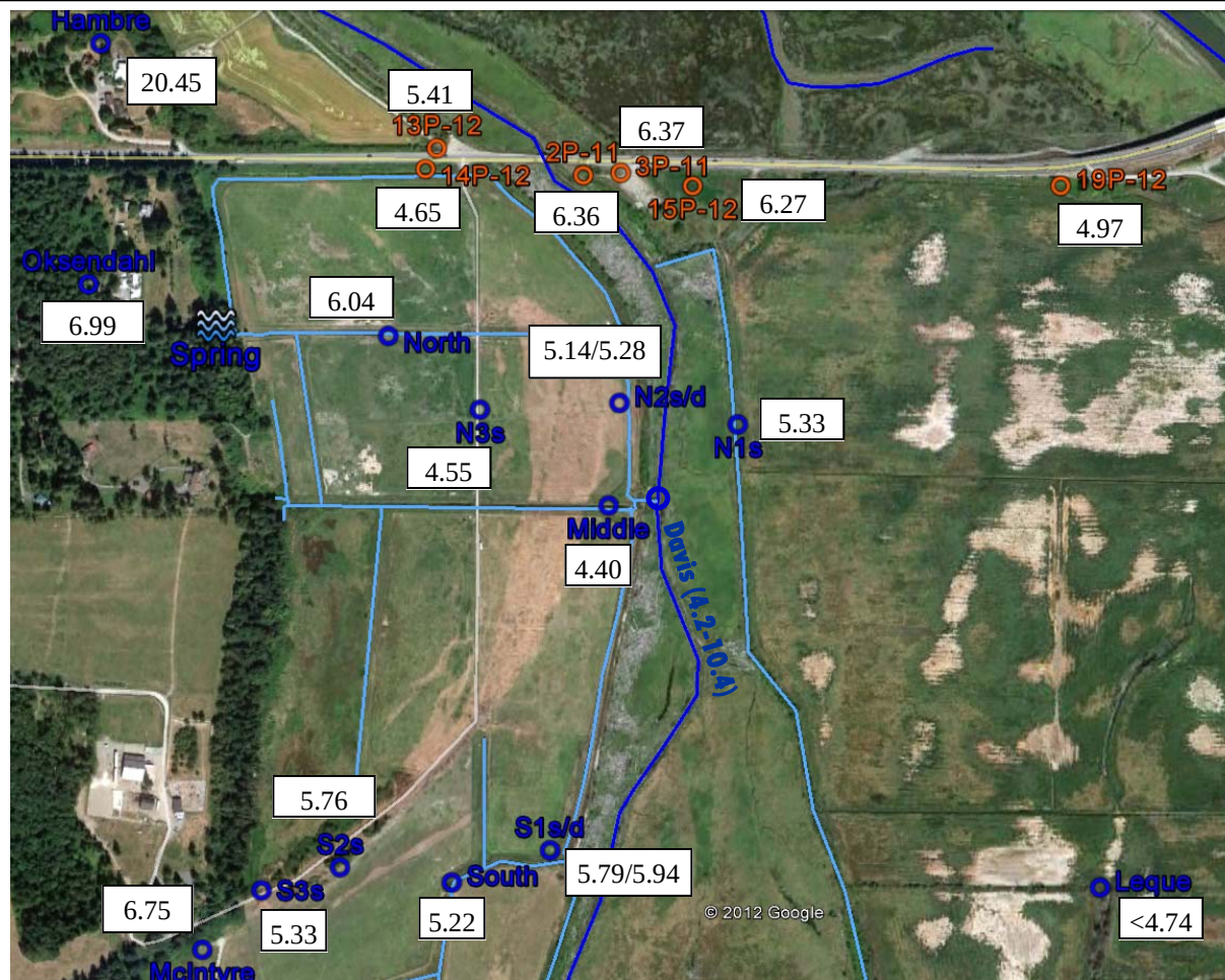
Figure B-5 Average Water Level Elevations for 3-Day Period Starting 9/4/12
