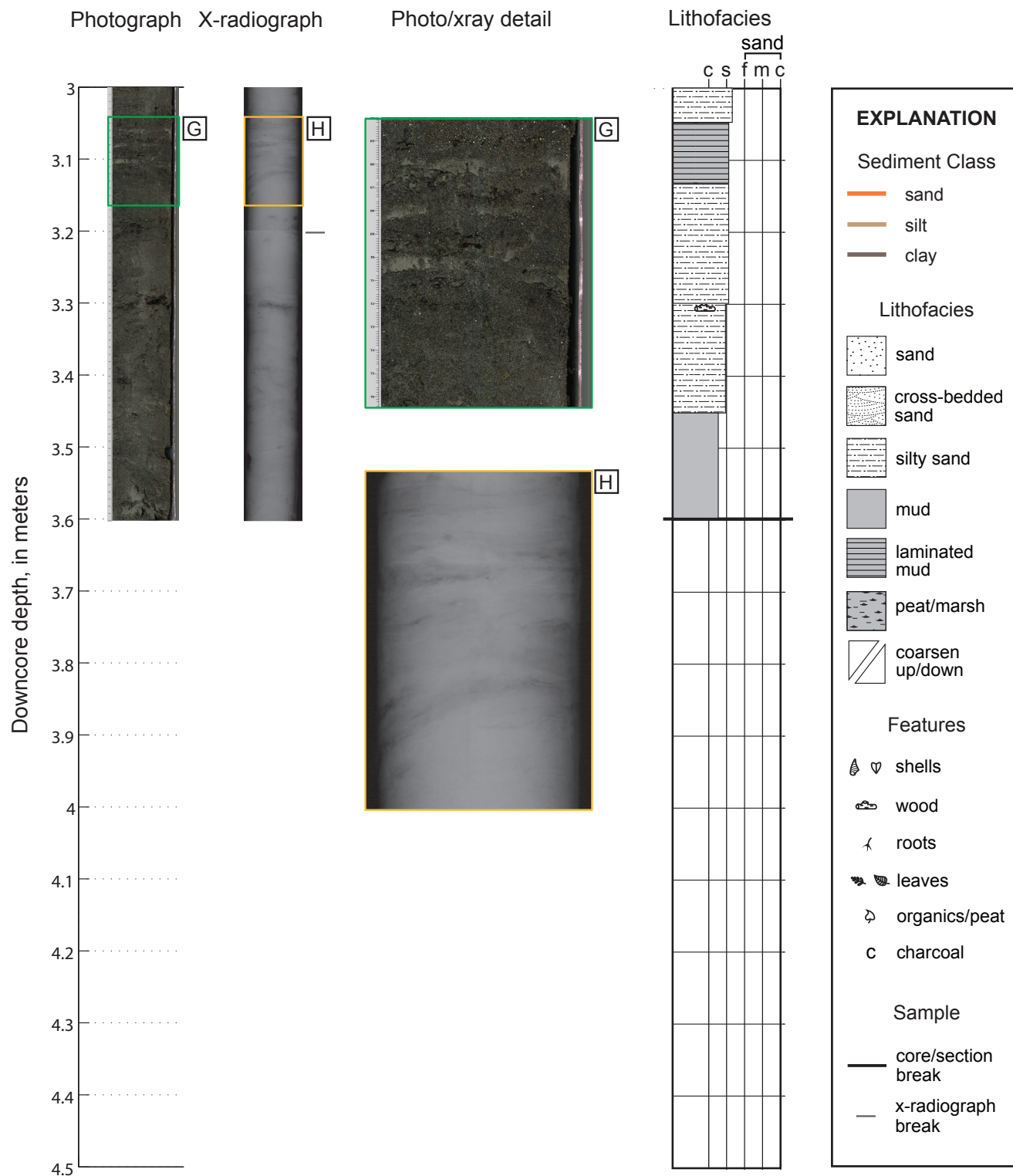
Figure A.1.9, cont.
