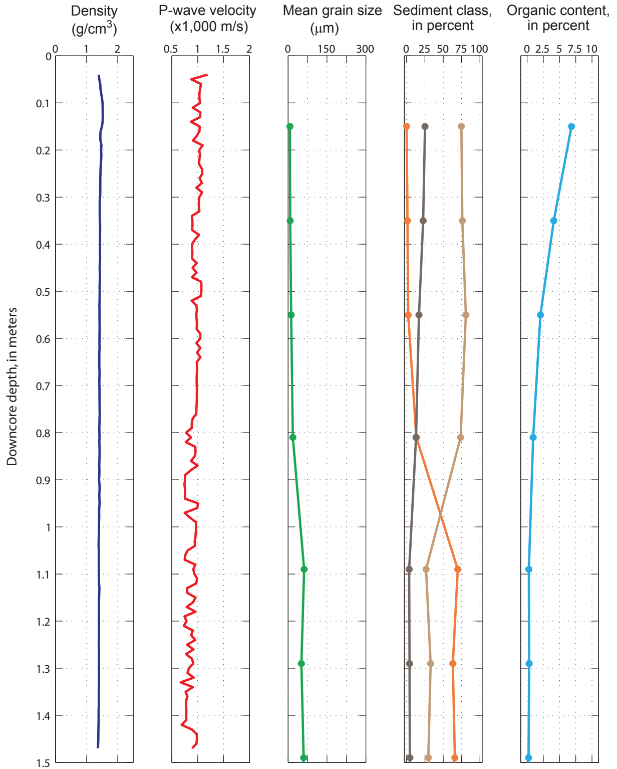
Figure A.1.11. Diagram of physical properties and lithology of sediments from Core C1, Skagit River Delta, Washington.
