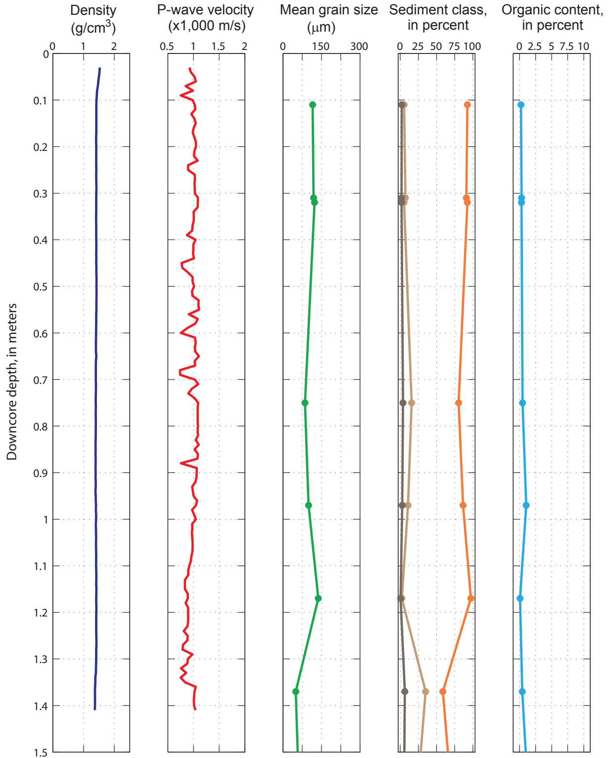
Figure A.1.10. Diagram of physical properties and lithology of sediments from Core B4, Skagit River Delta, Washington.
