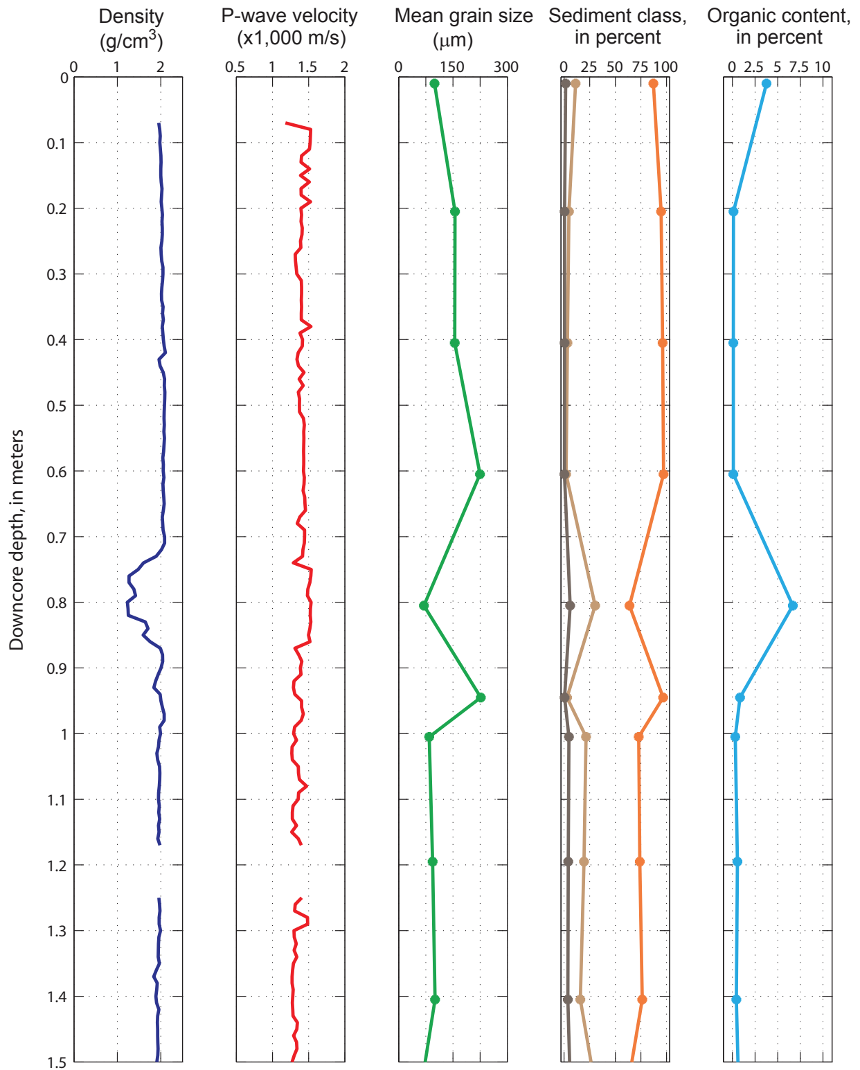
Figure A.1.6. Diagram of physical properties and lithology of sediments from Core A5, Skagit River Delta, Washington.
