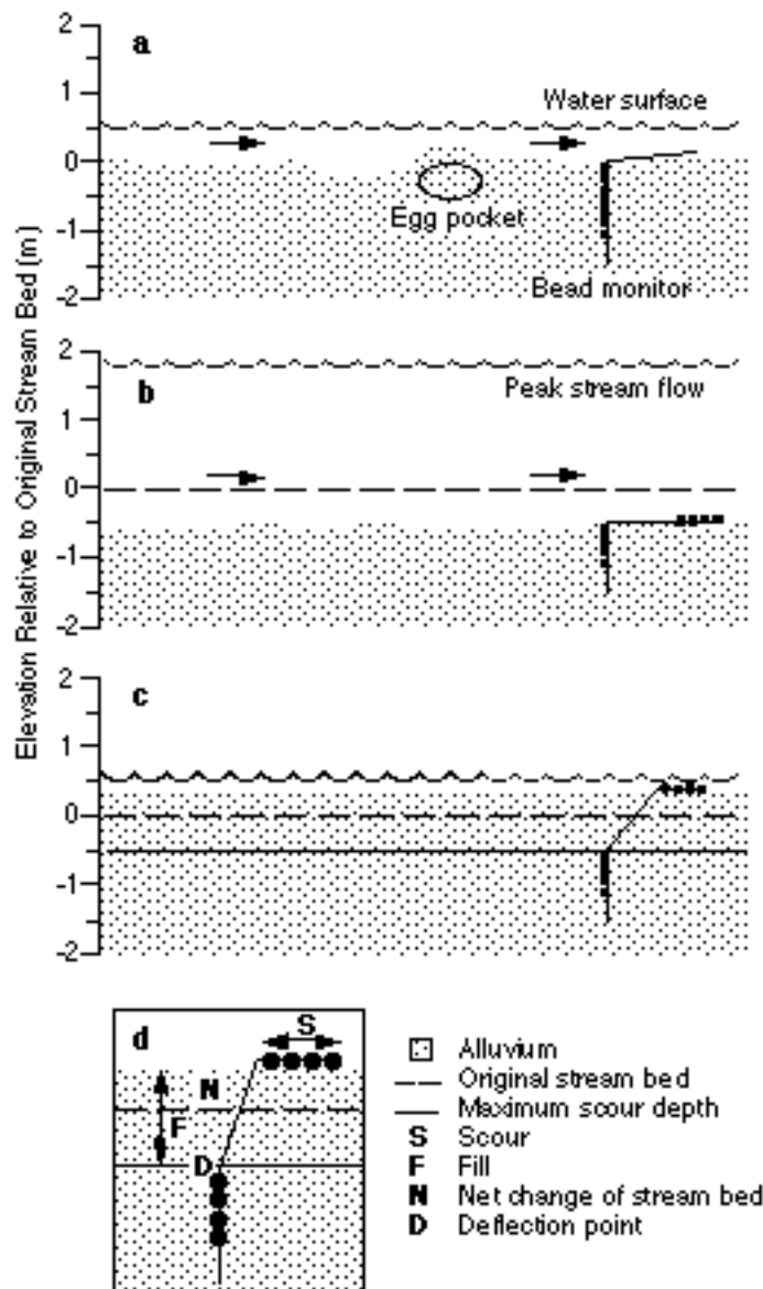
Figure 10b: Streambed scour and fill as measured by a sliding-bead scour monitor.
